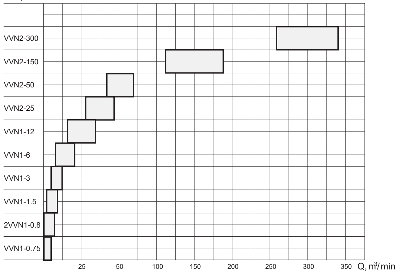
Pump Models
